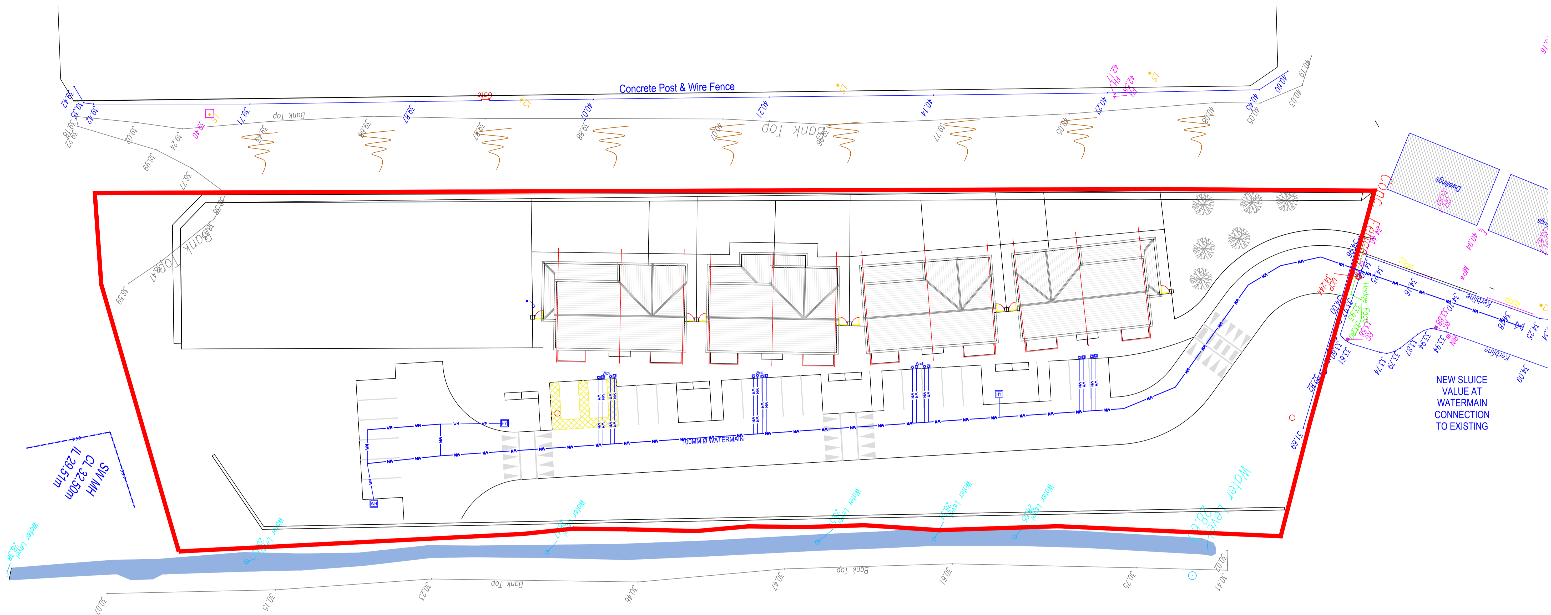
WATERMAIN LAYOUT SCALE 1:250
